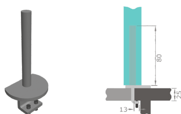
Spigot interference
